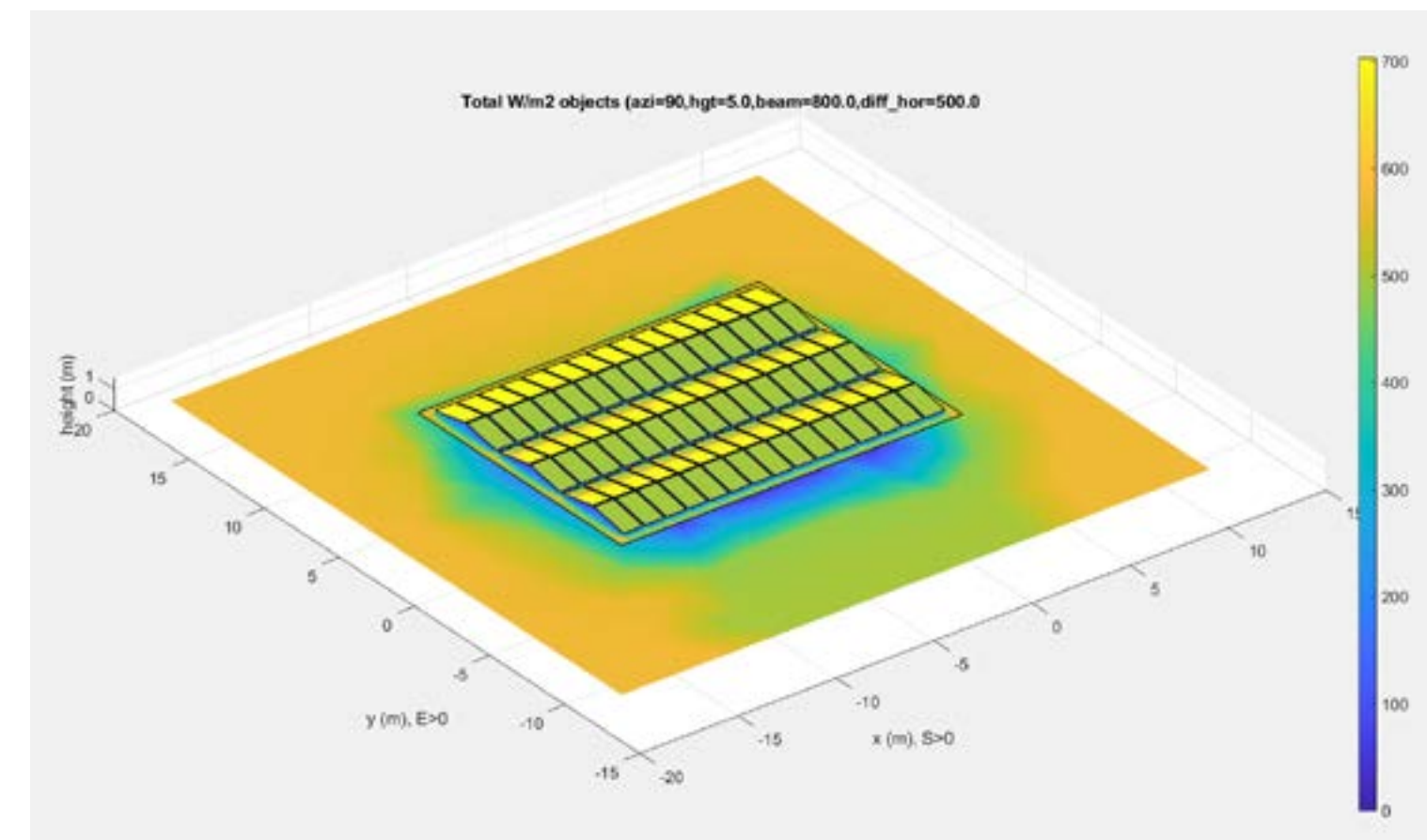
Simulation of energy performance of Floating PV
